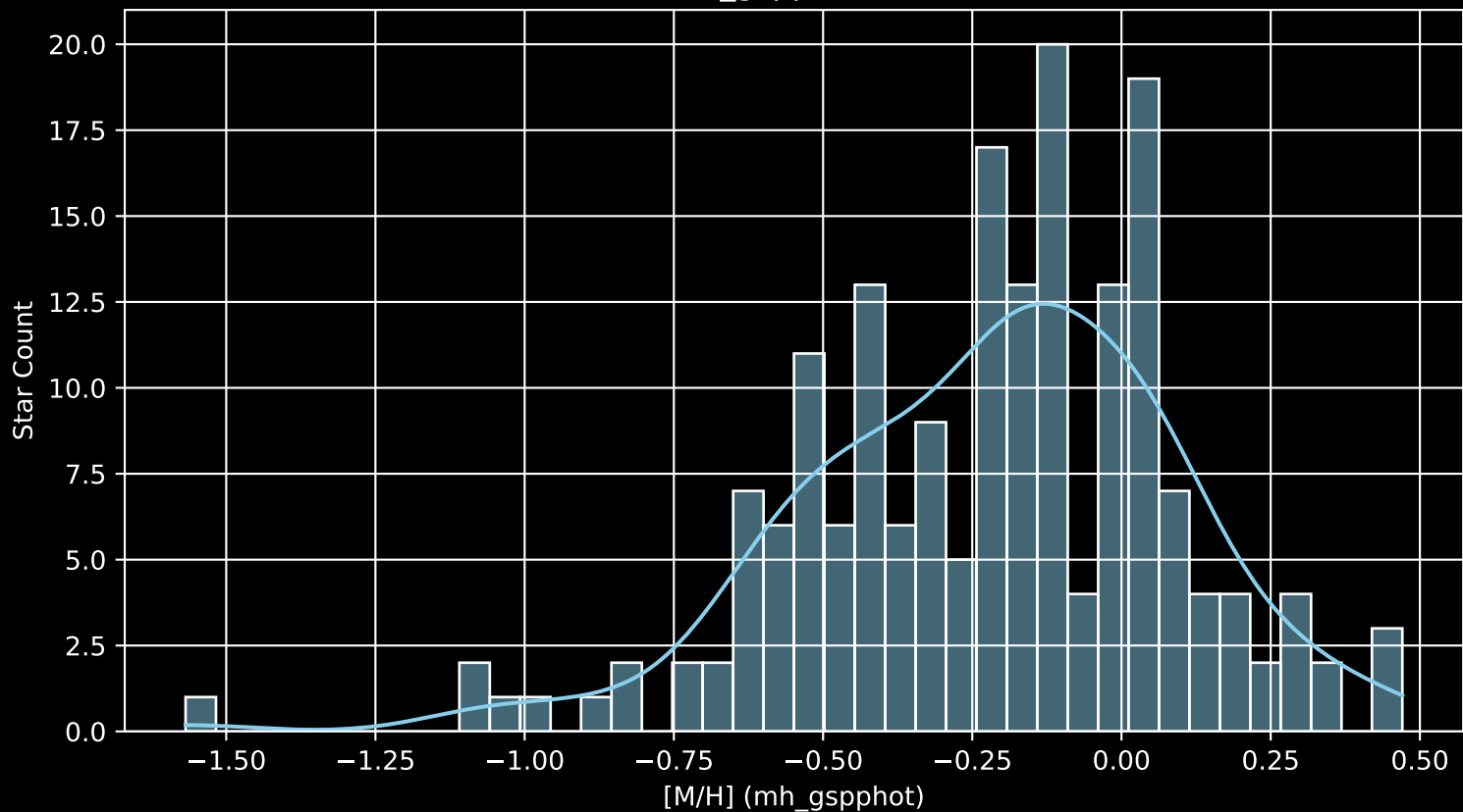
APOGEE DR17 Field: [045+89_MGA [M/H] (mh_gspphot) (n= 187)
