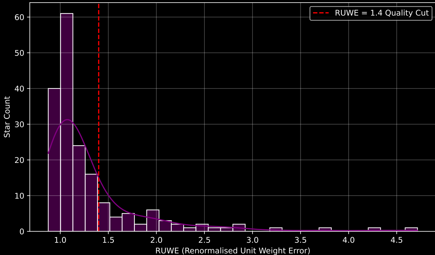
GAPOGEE DR17 Field [045+89_MGA] RUWE Distribution (n= 182)
