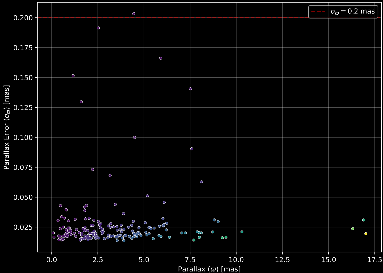
APOGEE DR17 Field: [045+89_MGA] Parallax Quality (n= 189)
