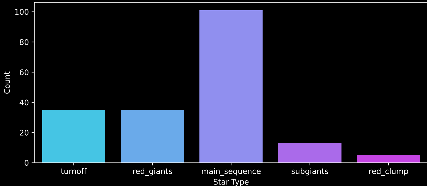
APOGEE DR17 Field: [045+89_MGA] Count plot of Star Type
