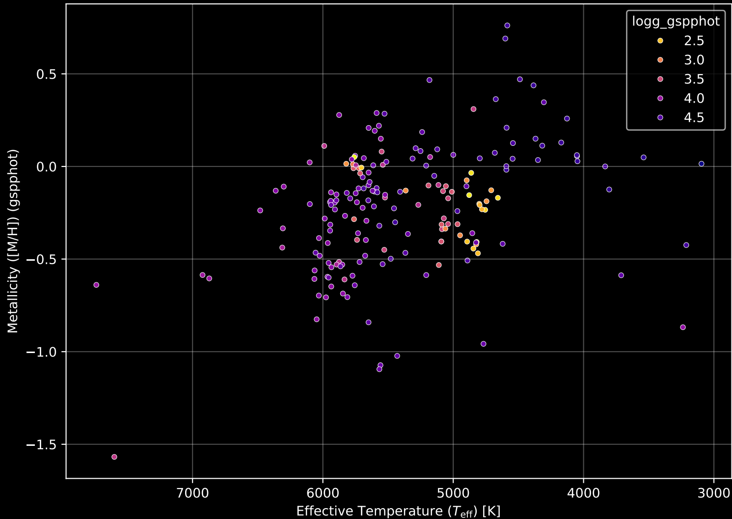
APOGEE DR17 Field: [045+89_MGA] Stellar Population Parameters (n= 189)
