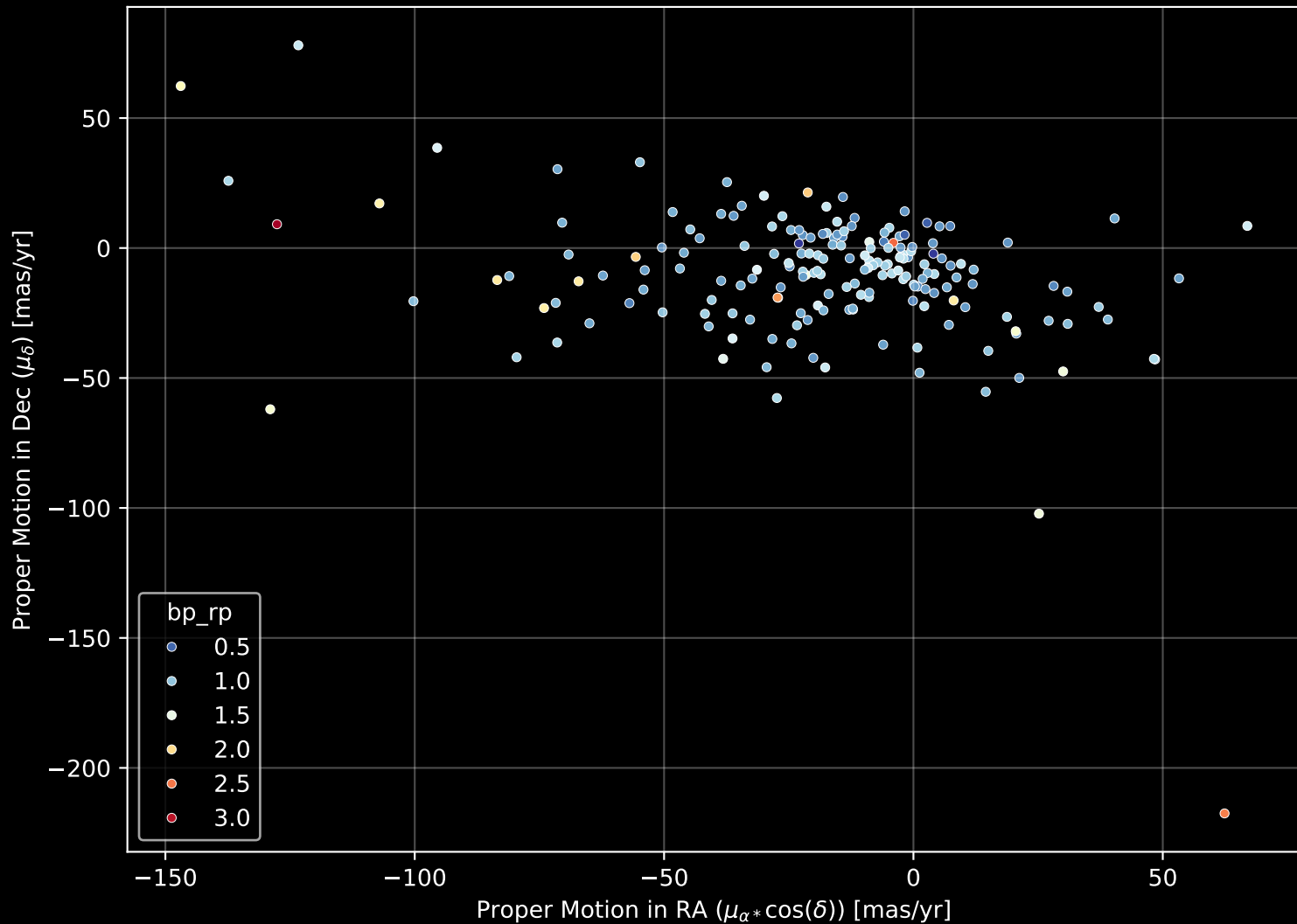
APOGEE DR17 Field: [045+89_MGA] Proper Motion Diagram (n= 189)
